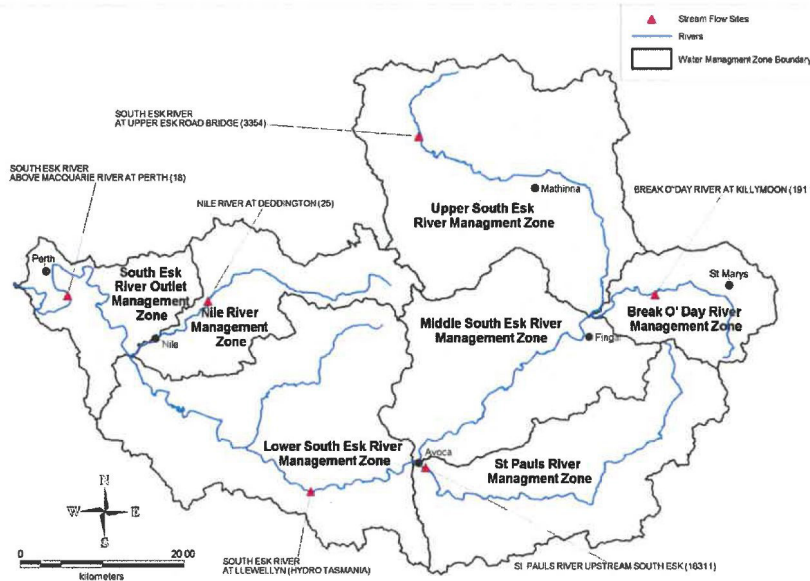
Figure 1. South Esk River Catchment
